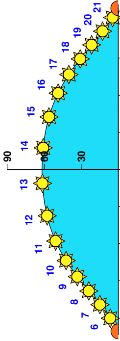
Sun elevation, for June 21
