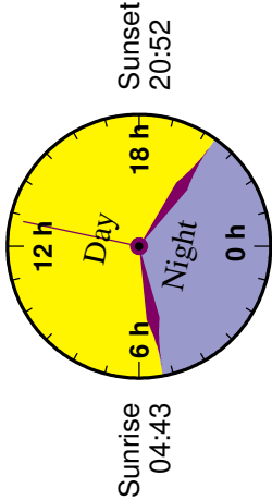
Duration of the day, for April 21
