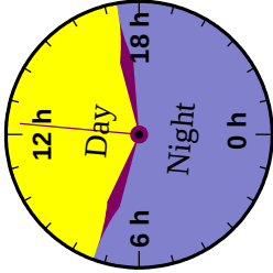
Duration of the day, for January 21
