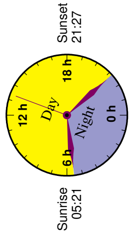
Duration of the day, for May 21
