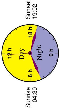
Duration of the day, for June 21
