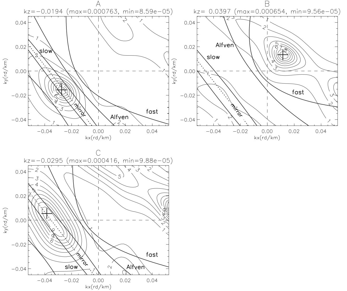
Figure 10. Same as Figure 7 for f_4 = 1.15 Hz. It shows the same behavior as the frequency f_3 for panels A and B, with a new maximum corresponding to mirror mode (panel C).
