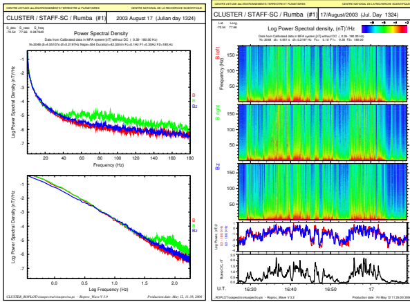
Fig. 4. Fourier spectra (left picture) and spectrograms (right picture) of magnetic fluctuations from STAFF-SC data in a MFA frame ( \delta B_z corresponding to \delta B_{||} ). The time resolution of the spectrogram is 4.55 s and the frequency resolution is 0.22 Hz. The lower cut-off frequency has been fixed at 0.35 Hz to get rid of any spin modulation effect (see text for more details).
