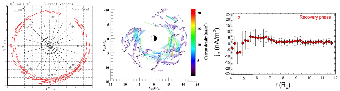
Figure 7. (left) Magnetic local time (MLT) scan of Cluster ring current (RC) passes, plotted in solar magnetic (SM) coordinates, and between -30^\circ to 30^\circ latitude (after Zhang et al., 2011). Averages (10 min) of the current density obtained from the curlometer are shown by the length and direction of each arrow. The measurements represent non-storm ( Dst > -30 nT) values of the RC. There is an overall increase in j_\phi from 03–12 MLT on the dawn-side while it remains low on the dusk side. (middle) Current densities projected into the ring plane are shown in a similar way (from THEMIS) for all storm activities during the recovery phase, showing the wider range of radial coverage achieved (for about 4–12 R_E ) and an enhanced current near midnight LT for storm events. (right) Radial profile of the current density from THEMIS measurements.
