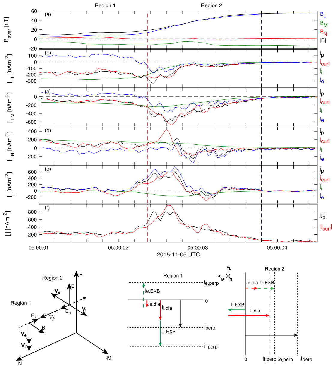
Figure 13. Top: Sources of a thin magnetopause current sheet calculated by MMS data. Bottom part: a schematic illustration of all the vectors. (left) The vectors of magnetic field B , electric field E , plasma velocity V , cross-field drift E \times B , and gradient of pressure \nabla p in regions 1 and 2 and (middle and right) current distribution in region 1 and region 2. Note that region 1 and 2 here refer to the outer and inner magnetopause current sheet region, respectively. The Figure is adopted from Dong et al. (2018).
