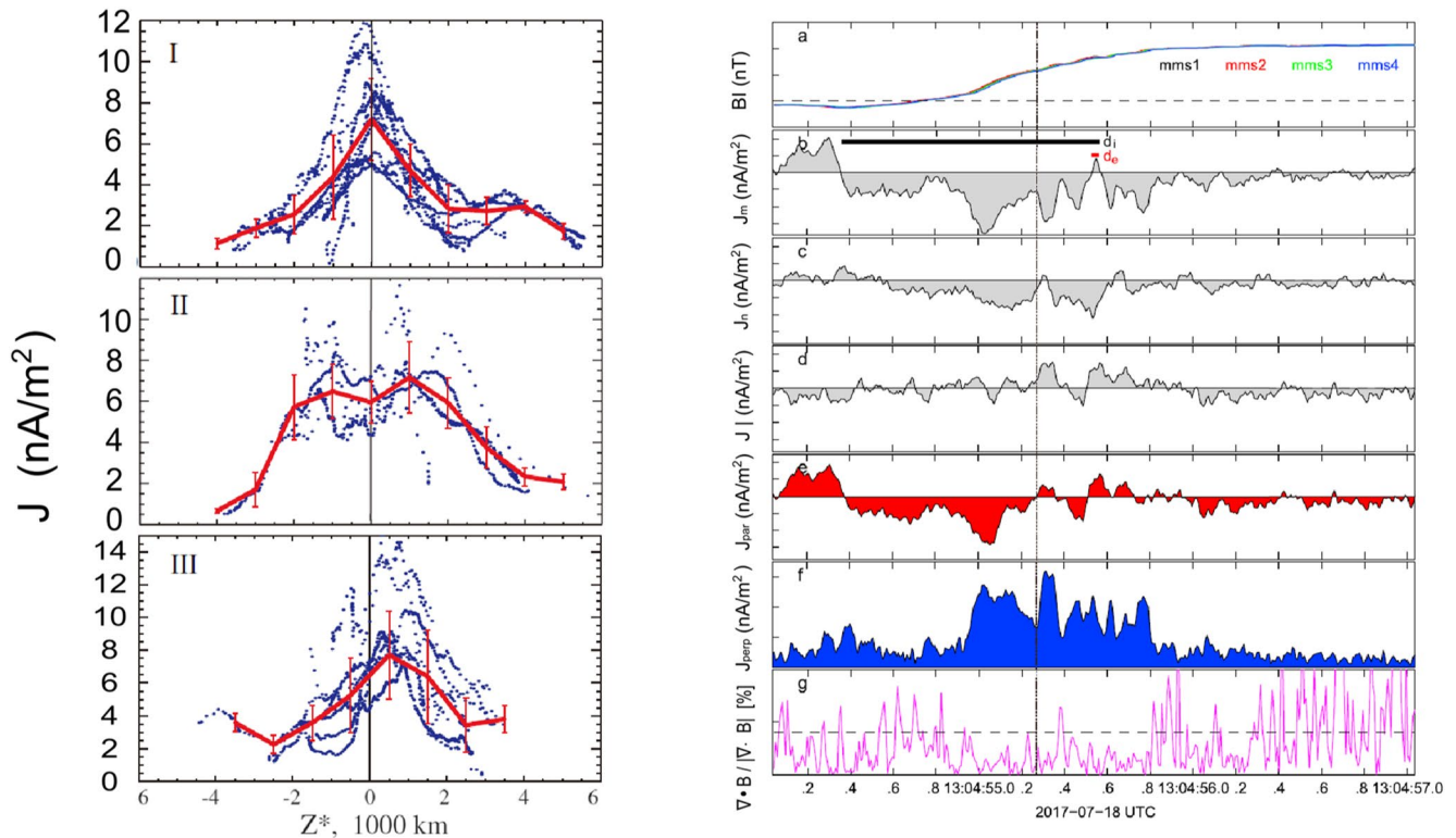
Figure 8. (left) Dependence of the magnetotail current |J| in \text{nA/m}^2 on the distance above and below the neutral sheet for individual crossings (blue dots) and binned averages (red lines). The data are classified as three different characteristic types of current sheet (from Runov et al., 2006). (right) MMS observation of the structure of J on electron-scales around a DF in boundary normal coordinates. The top four panels show the 4-spacecraft B_i magnetic field components and the current density (as N,M,L components). Local inertial lengths for ions and electrons is indicated as black and red bars in panel (b). Panels (e) and (f) show the parallel/perpendicular J components. Panel (g) shows the Q parameter. The high-density to low-density boundary across the DF layer is indicated by the black dashed line (adapted from Liu et al., (2018)).
