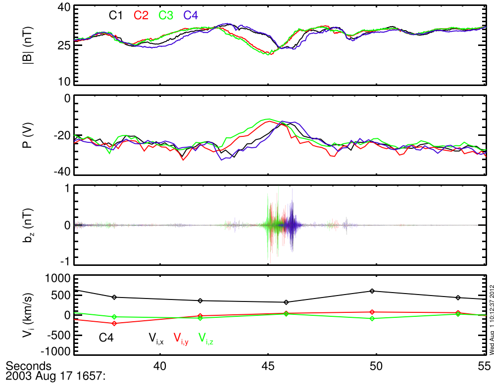
Figure 4. Case 2. (top to bottom) the magnitude of the magnetic field |B| (FGM); the spacecraft potential (EFW); the z component of the high-frequency magnetic field fluctuations b_z measured by each spacecraft (STAFF SC); the three components V_{i,x} , V_{i,y} , and V_{i,z} of the ion velocity (black, red, and green color, respectively (CIS-CODIF)).
